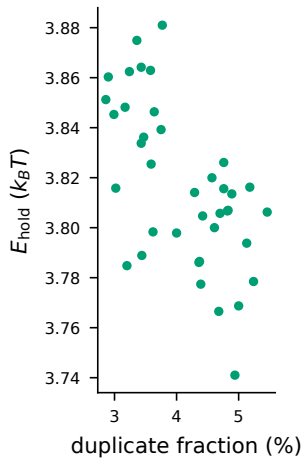
b charr: \rho = -0.57
