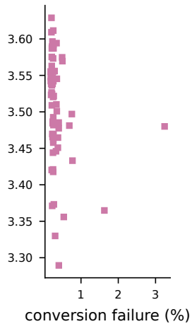
c salmon: \rho = -0.38
