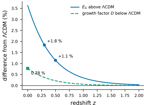
b Growth falls, lensing ( \Sigma = 1 ) does not
