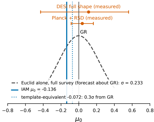
a \mu_0 = -0.136 against present and forecast widths
