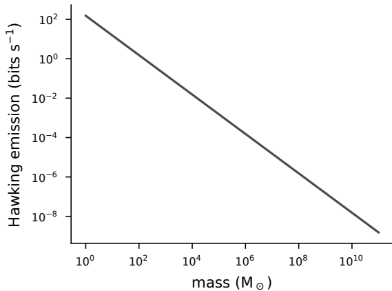
b \Gamma = c^3/(1920 GM \ln 2)
