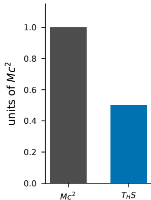
c Horizon: Mc^2 = 2T_H S
