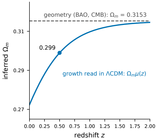
a Growth and geometry give different \Omega_m
