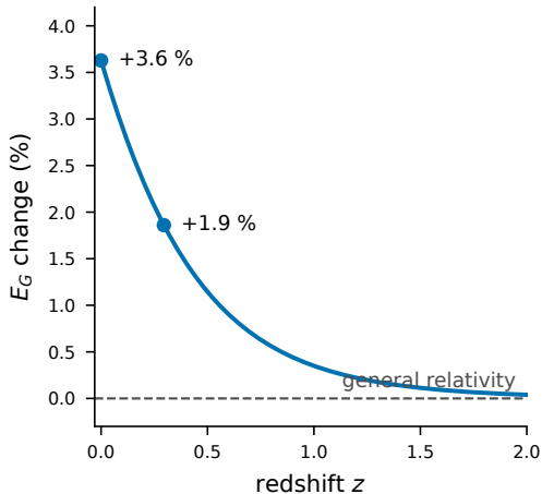
b E_G lies above general relativity
