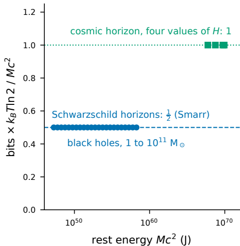
a A horizon's bits cost half its rest energy
