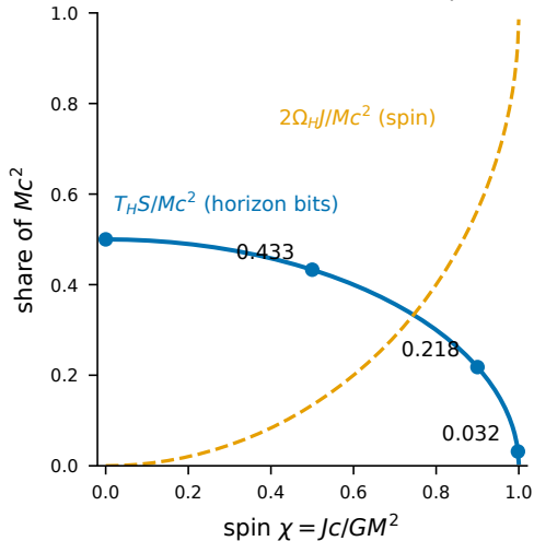
b Rotation moves the half into spin
