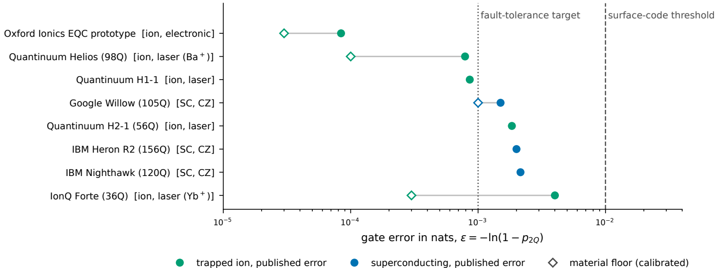
Published two-qubit errors against the error-correction scale and the material floors
