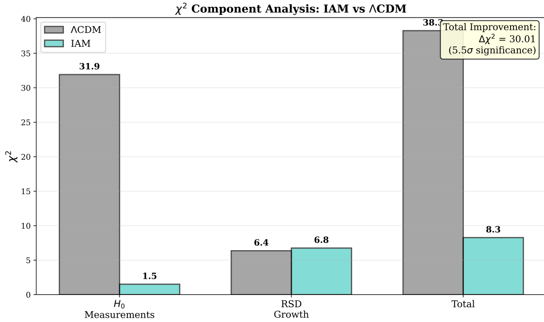
Figure 7: \chi^2 Component Analysis showing H_0 measurements dominate the improvement. IAM reduces \chi^2_{H_0} from 31.9 to 1.5 while maintaining DESI fit quality. Total improvement: \Delta\chi^2 = 30.01 (5.5 \sigma ).
