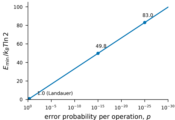
a Reliable switch: E_{\min} = k_B T \ln(1/p)
