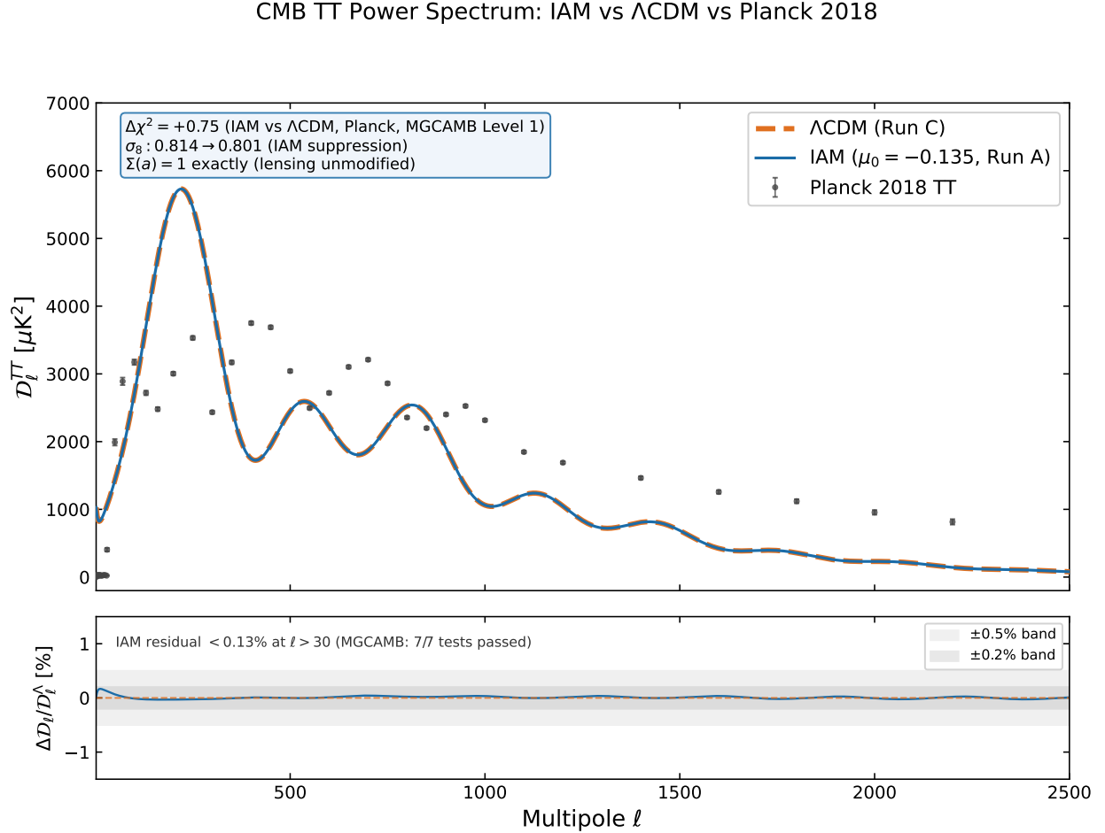
Figure 2: CMB TT power spectrum for IAM (Run A, solid blue) and \Lambda CDM (Run C, dashed orange), computed from MGCAMB Level 1 posterior mean parameters and compared against Planck 2018 bandpowers. The residual panel shows the fractional difference is < 0.13\% at \ell > 30 , consistent with the dual-sector prediction that \beta_\gamma \approx 0 leaves the photon sector unmodified. The \Delta\chi^2 = +0.75 penalty relative to \Lambda CDM is within the expected range for a one-parameter modification constrained by the same data.
