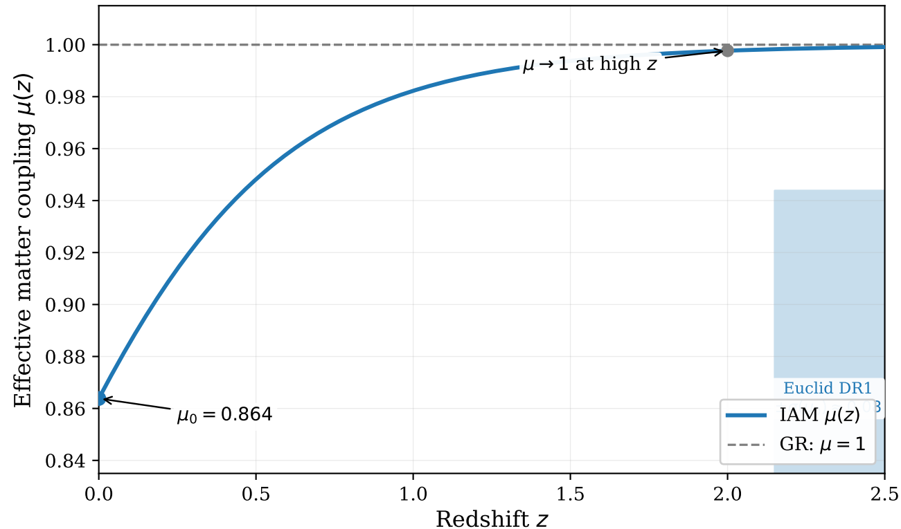
IAM matter-sector coupling: late-time suppression from \beta_m E(a) friction term
