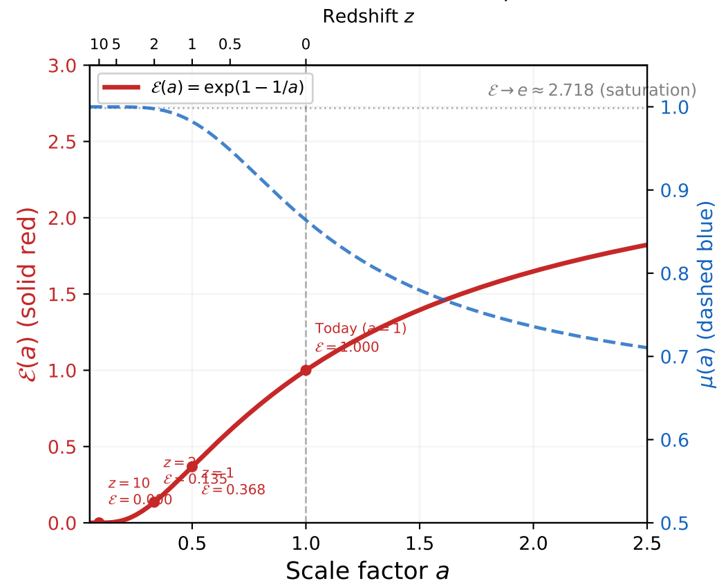
(c) Activation Function & \mu(a)
