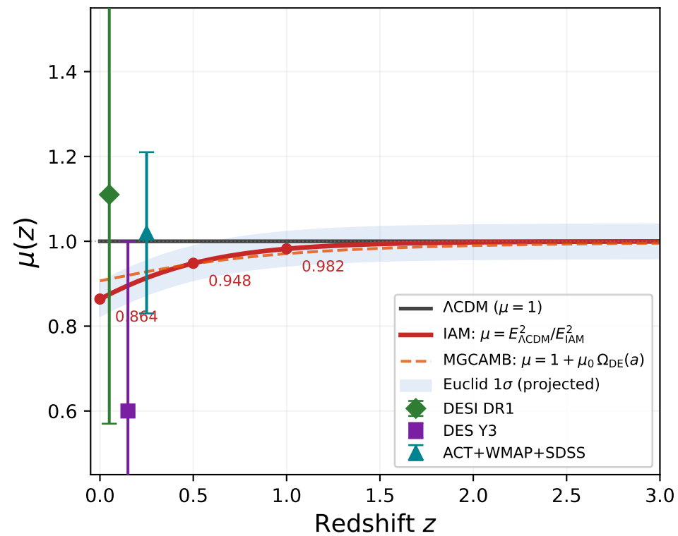
(a) Gravitational Coupling \mu(z)
