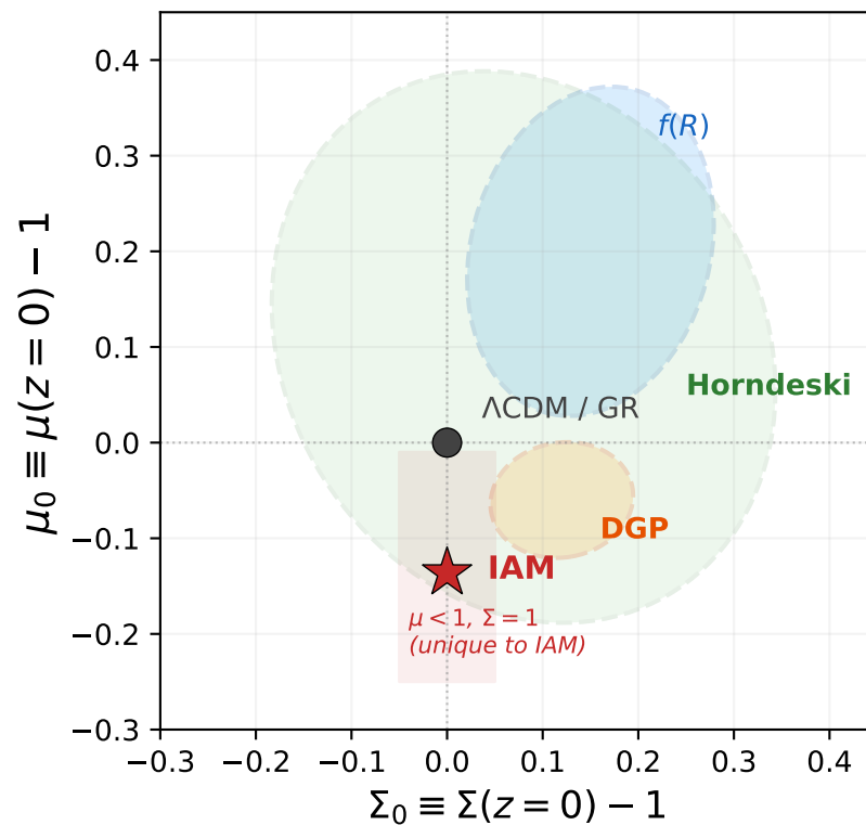
(b) \mu - \Sigma Phase Space
