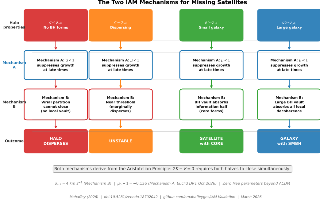
Figure 2: The unified mechanism across four halo regimes. The Aristotelian Principle requires both halves of the virial partition to close simultaneously. Mechanism A ( \mu < 1 , confirmed by 17 MCMC chains) reduces growth at late times for all halos. Mechanism B (dispersal condition) imposes a threshold below which no halo can virialize. Both mechanisms share the same physical origin: 2K + V = 0 at every scale.
