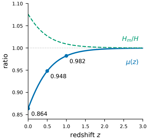
b Matter feels the record term late
