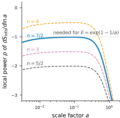
a p = -1 in the matter era only for n = 7/2
