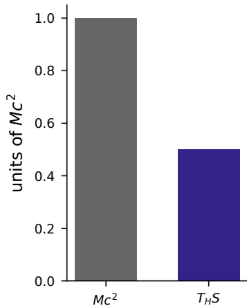
c Horizon: Mc^2 = 2T_H S
