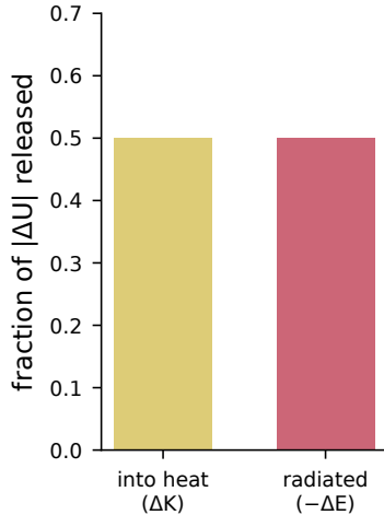
b Contraction: half and half
