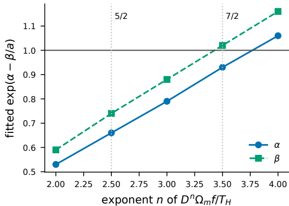
a The cosmology wants n \approx 3-4
