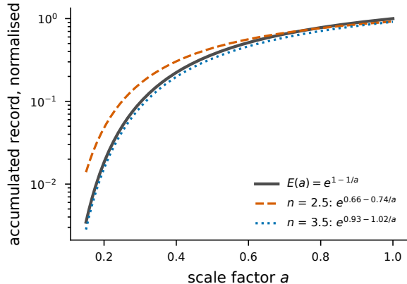
b 5/2 does not reproduce the activation
