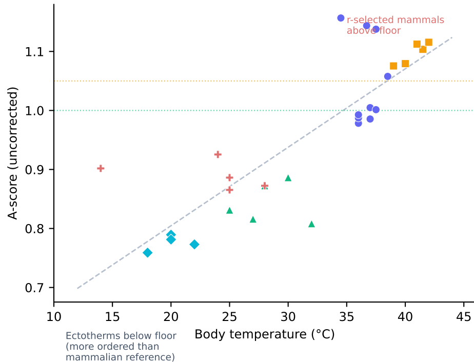
Raw A-scores vs body temperature r = +0.835 , p = 1.8\text{e-}08
