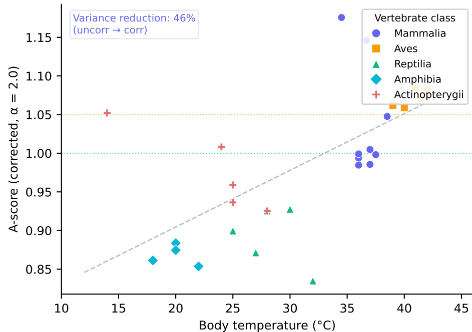
Temperature-corrected A-scores r = +0.627 , p = 2.7\text{e-}04
