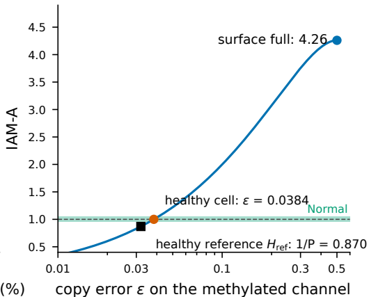
b Molecules: IAM-A up to the full surface, 4.26
