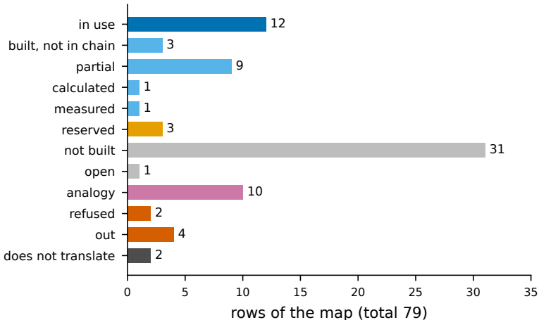
The 79-row map scored against chain v3
