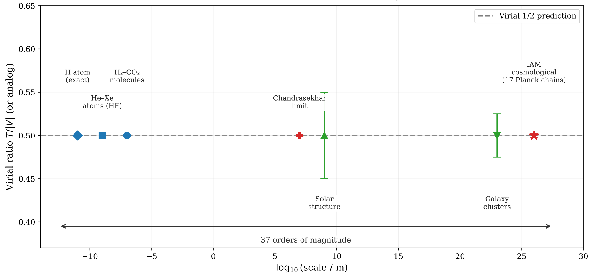
The 1/2 partition across 37 orders of magnitude
