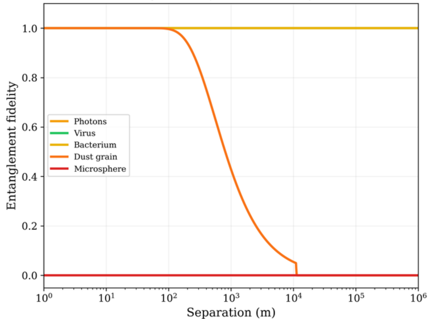
(a) Entanglement Survival vs Distance ( T=10 mK, matter at 1 m/s)
