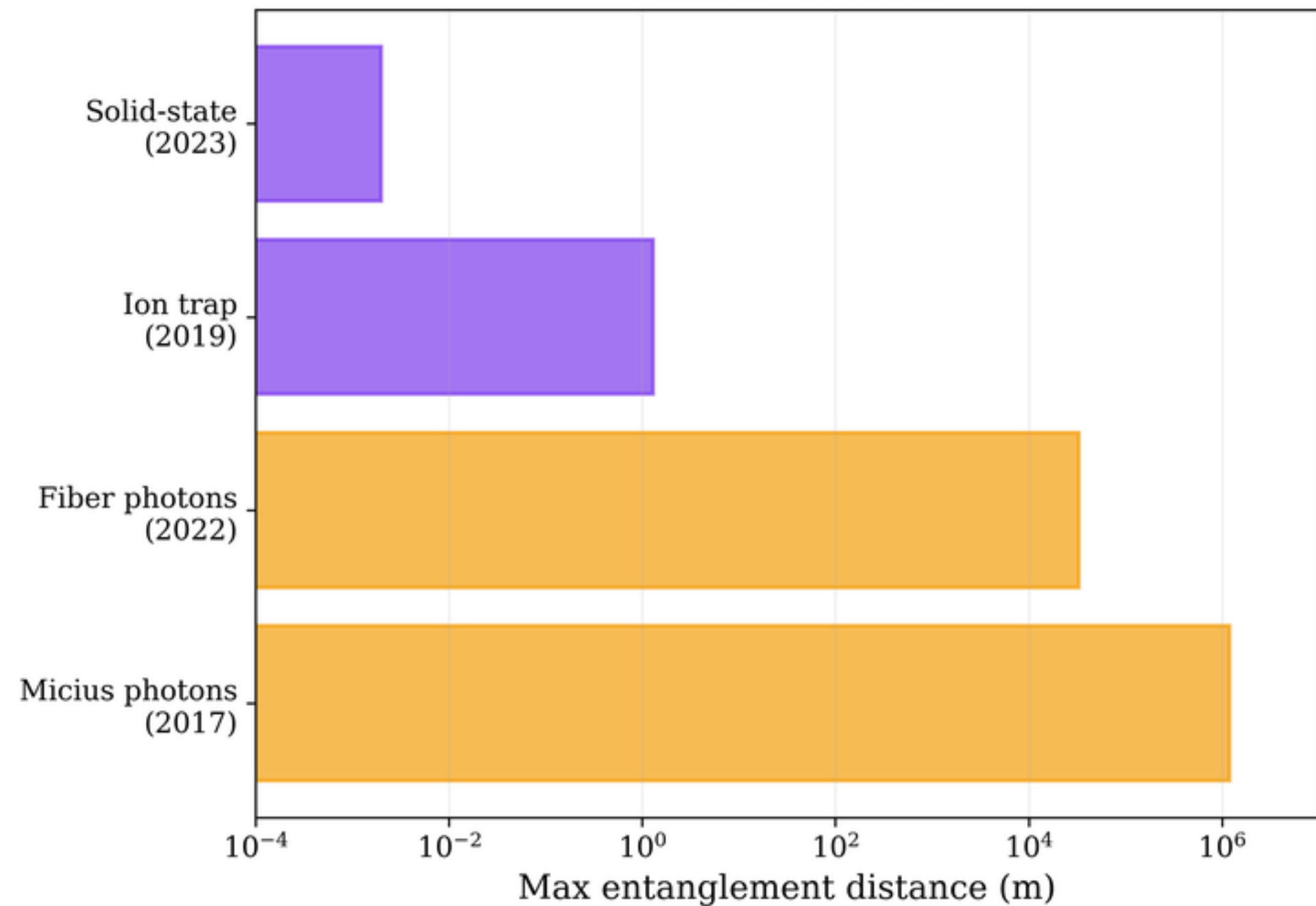
(b) Distance Records: Photons vs Matter
