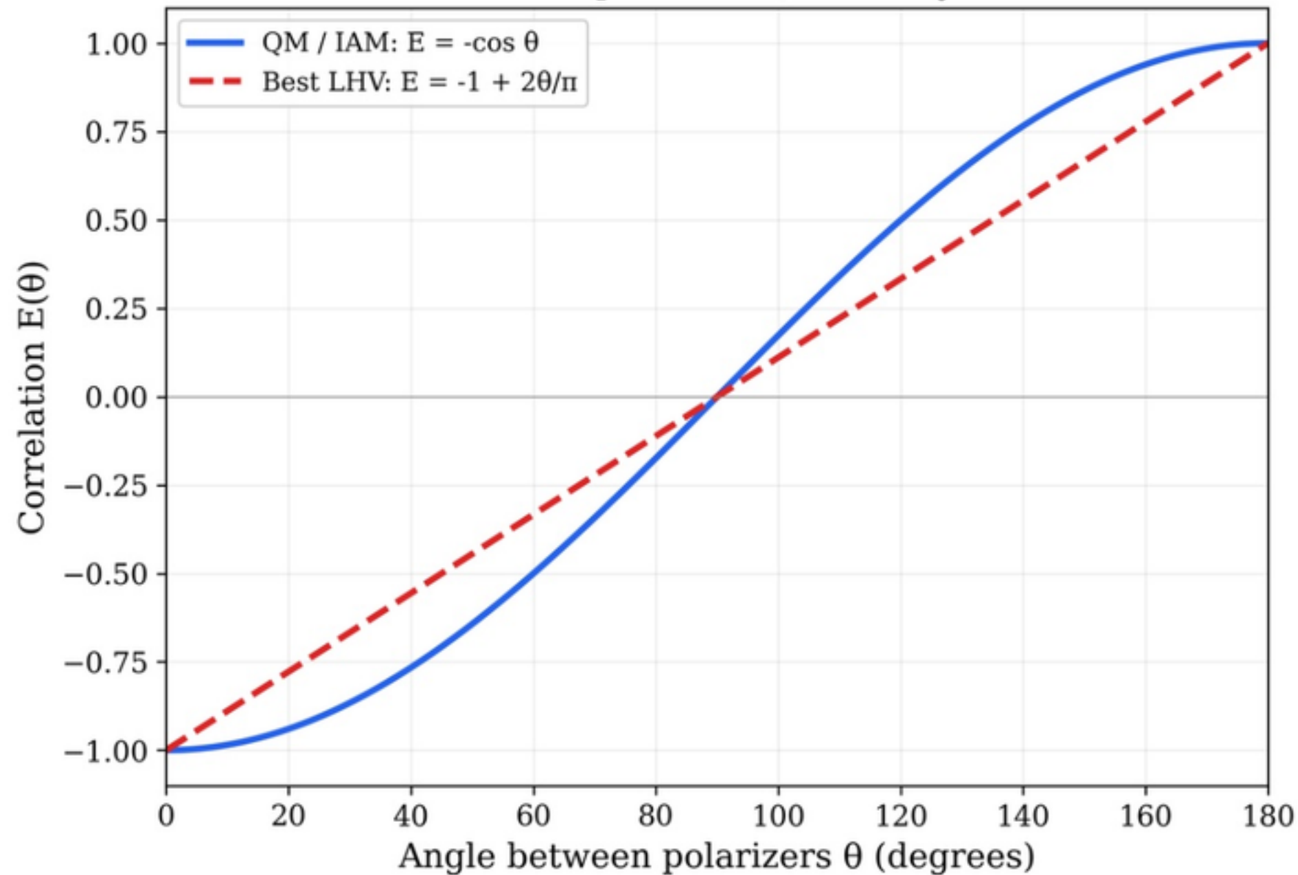
(a) Bell Correlation Function IAM reproduces QM exactly
