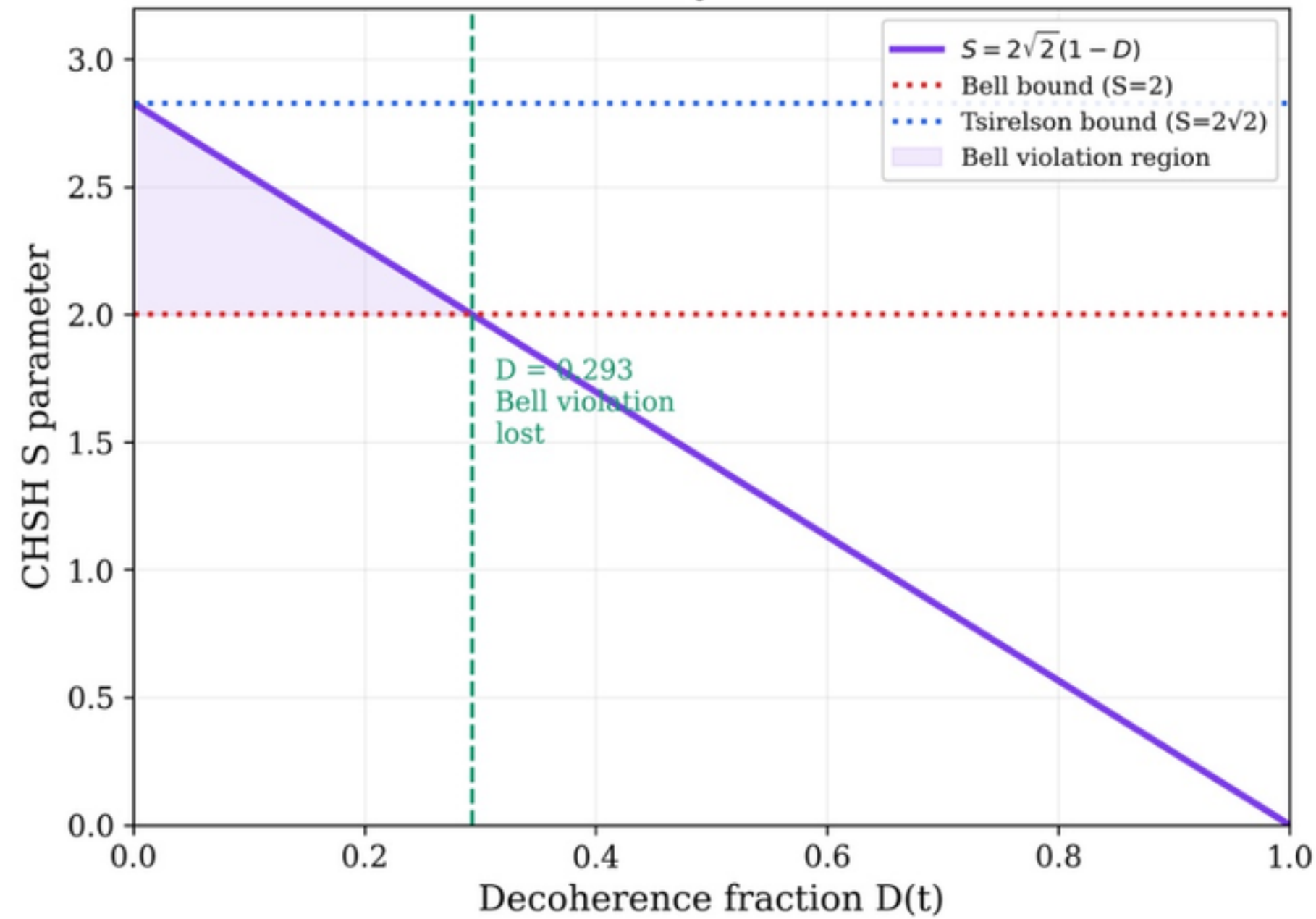
(b) Matter Entanglement: Bell Violation Decays with Decoherence
