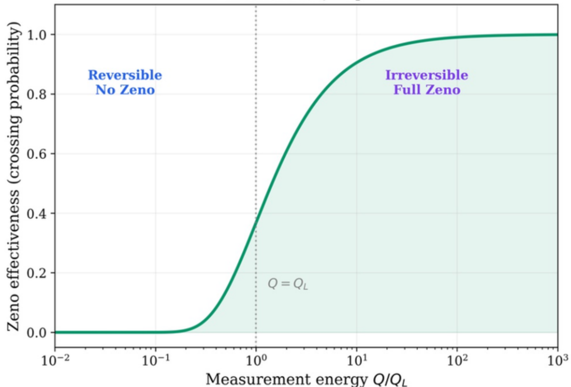
(b) Zeno Effectiveness vs Measurement Strength Threshold at Q = k_B T \ln 2
