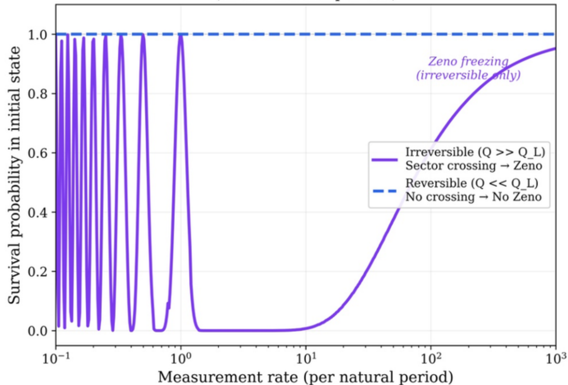
(a) Quantum Zeno Effect (after 5 natural periods)
