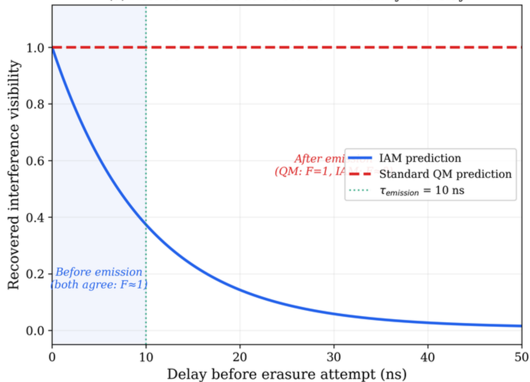
(a) Atomic Which-Path Detector: Visibility vs Delay
