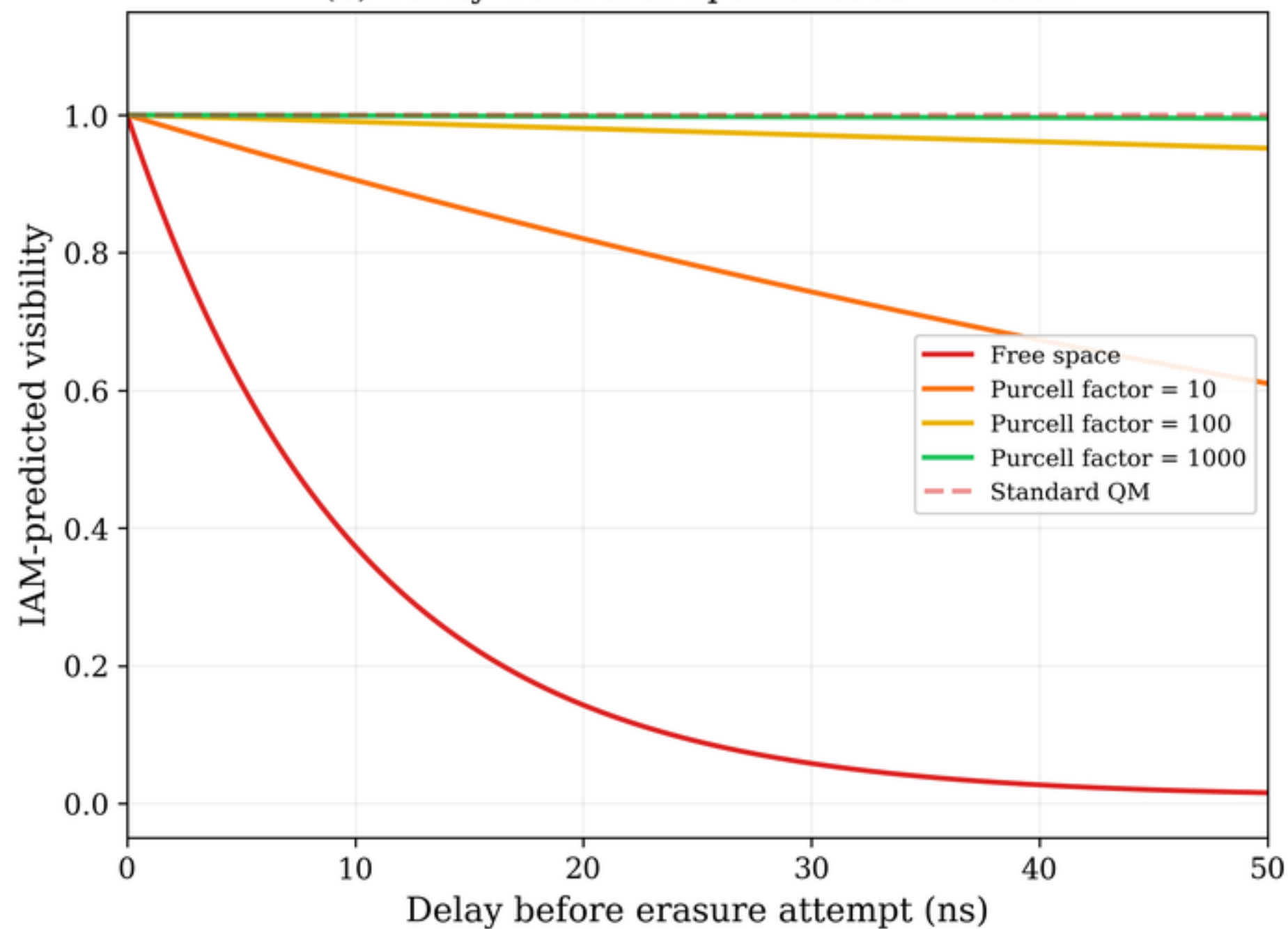
(b) Cavity Control of Spontaneous Emission
