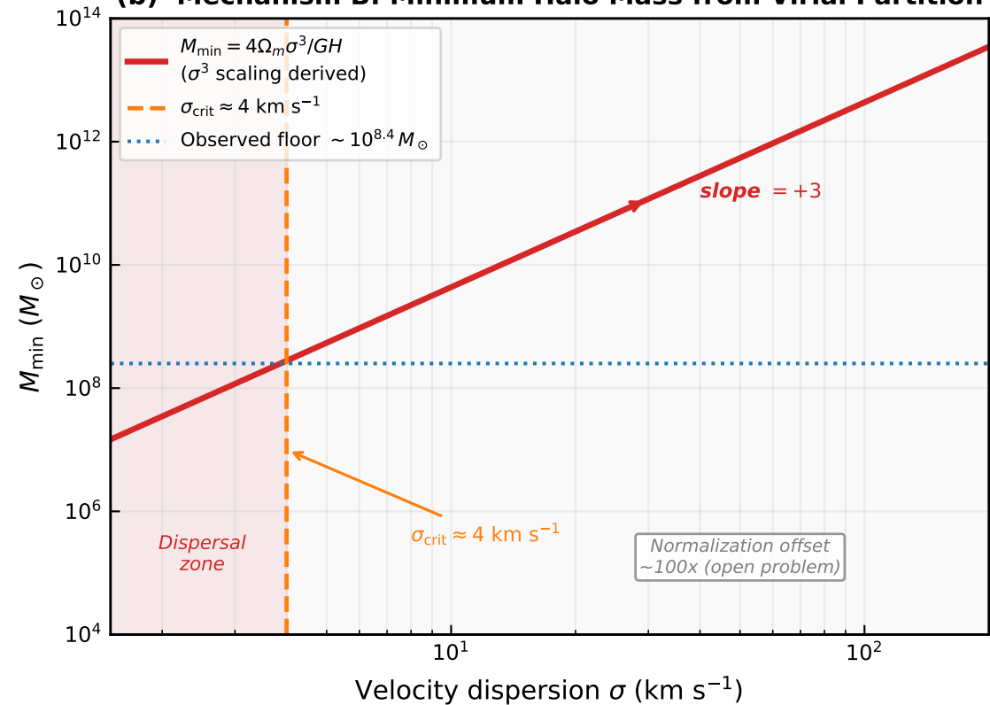
(b) Mechanism B: Minimum Halo Mass from Virial Partition
