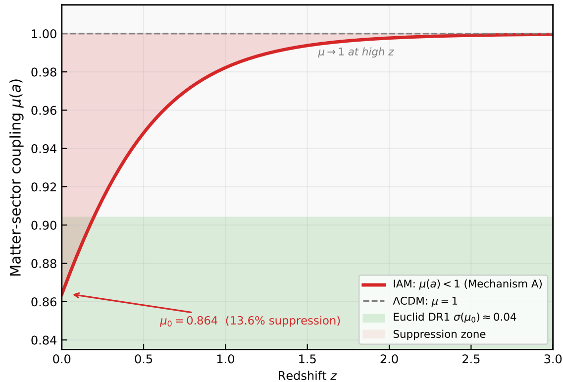
(a) Mechanism A: Growth Suppression from \mu < 1
