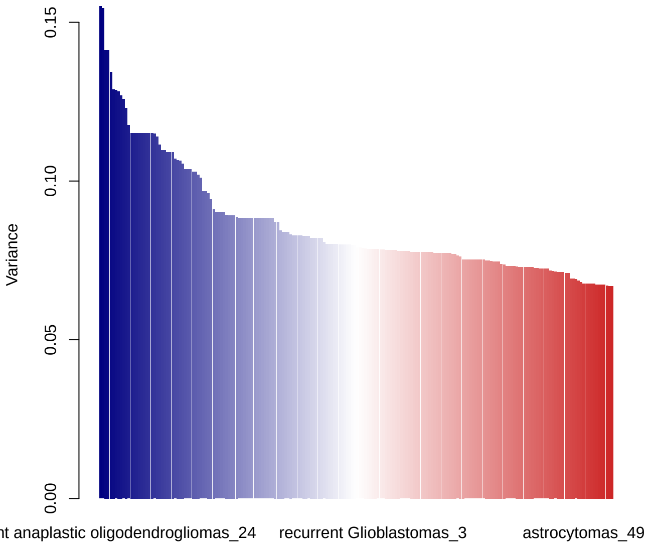
Top 200 most variable pathways
