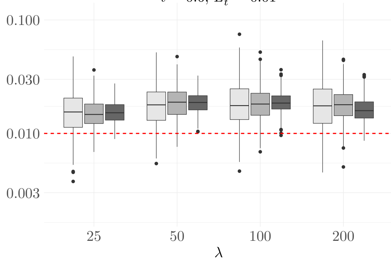
t = 0.6, L_t^2 = 0.01
