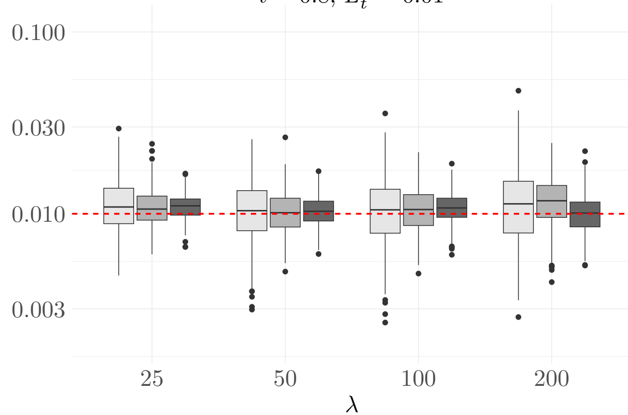
t = 0.8, L_t^2 = 0.01
