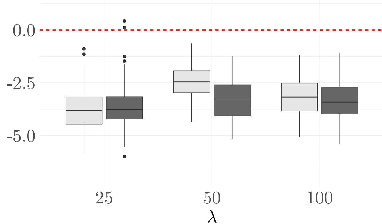
(c) ISE ratio w.r.t. RP20 under \mathcal{T}_{n_0}^{1/2}
