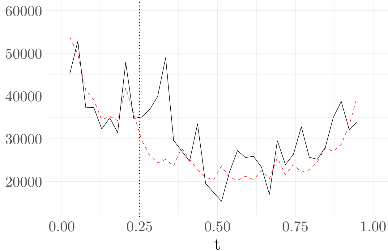
(c) Facebook stock volume \mathcal{T}_{n_0}^{3/4}
