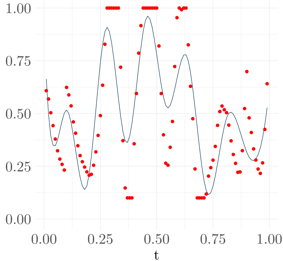
\hat{H}_t - Pointwise and smoothed curve
