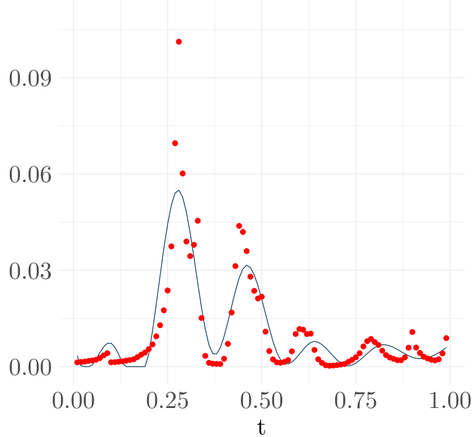
\hat{L}_t^2 - Pointwise and smoothed curve
