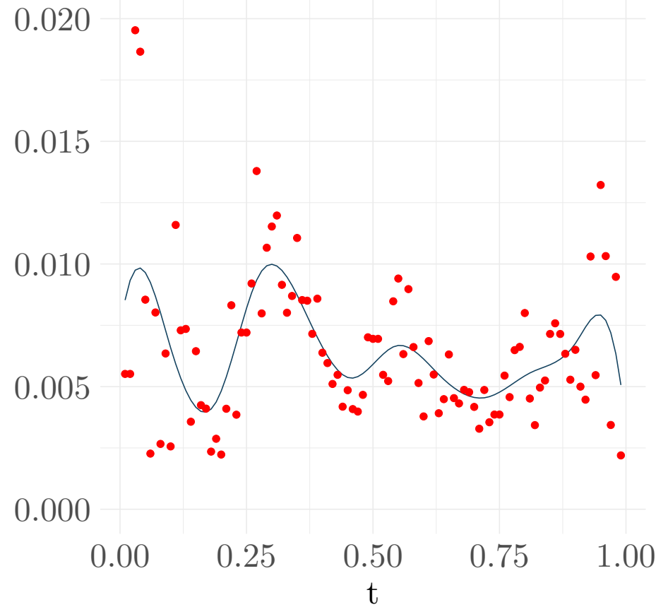
\hat{\sigma}(t) - Pointwise and smoothed curve
