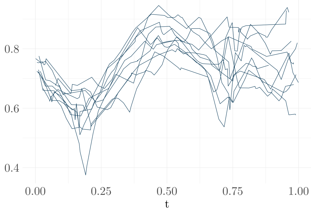
\{Y_{n,i}\} - \lambda = 50 - Innov + \mathcal{N}(0, \sigma^2 = 0.01) - 10 last curves
