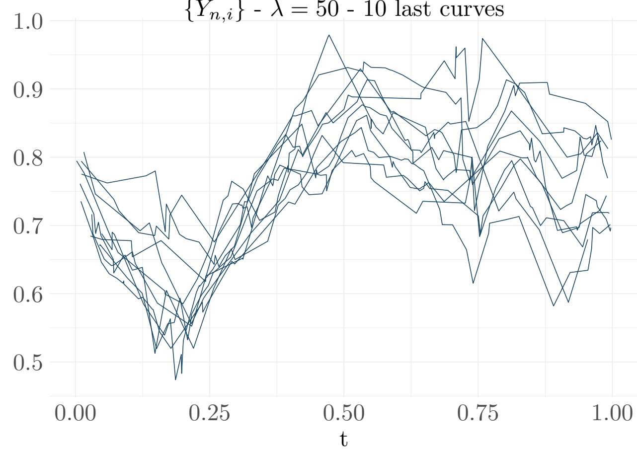
\{Y_{n,i}\} - \lambda = 50 - Innov + \mathcal{N}(0, \sigma^2 = 0.01) - 10 last curves
