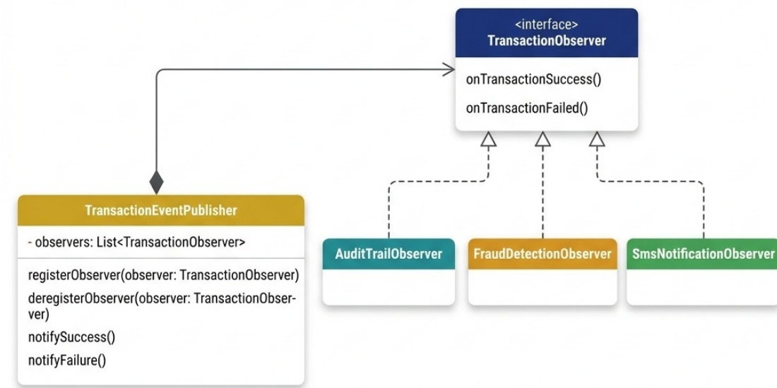
Figure 7.1: Observer Pattern Class Diagram
