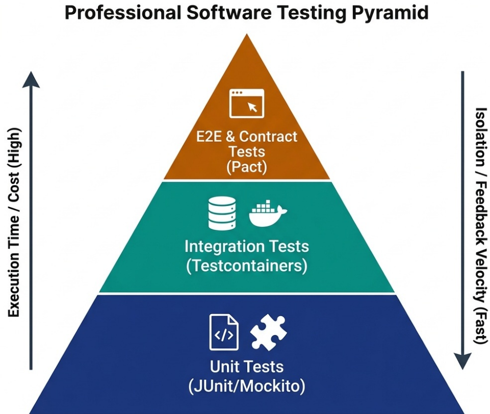
Figure 20.1: The Technical Testing Pyramid
