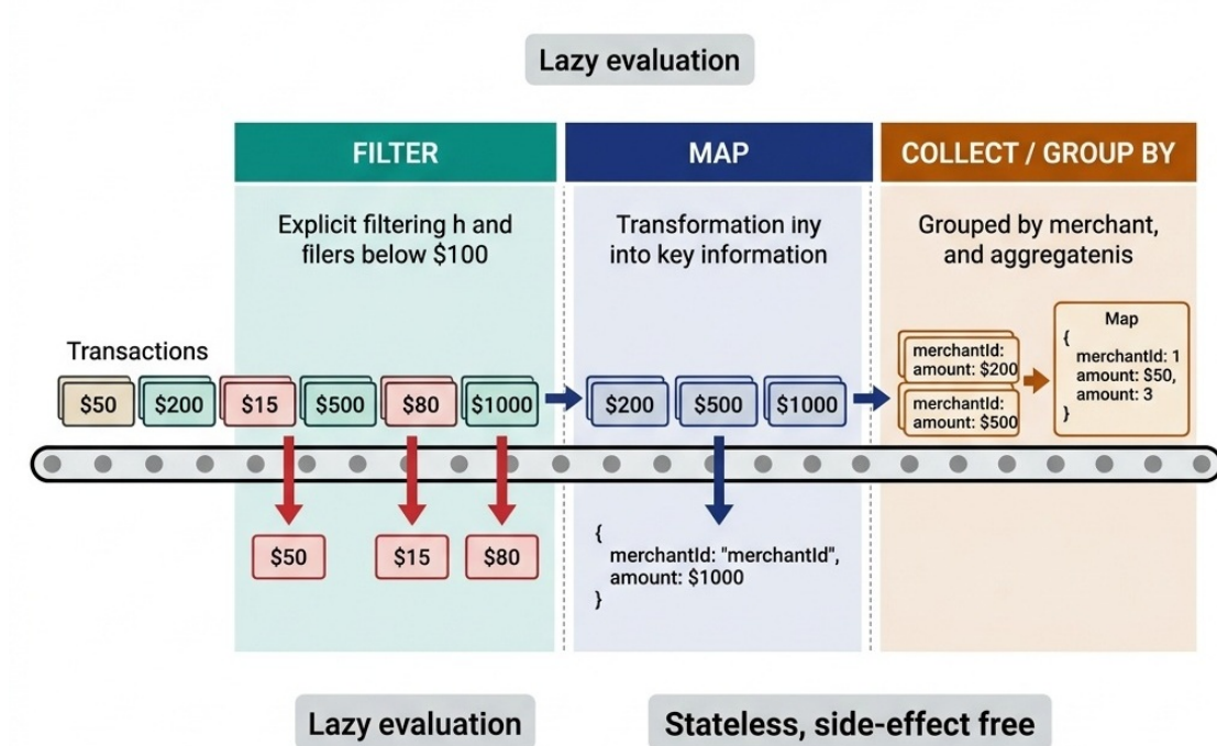
Figure 6.1: Stream Pipeline Visualization
