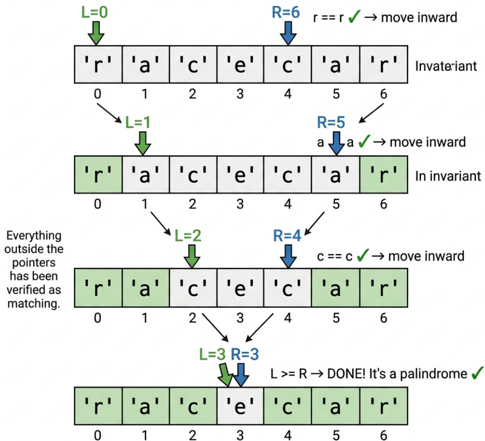
Figure 10.2: Two-Pointer Convergence — Palindrome Verification
