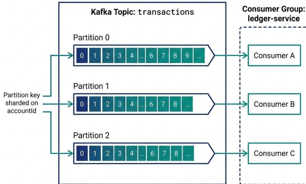
Figure 20.1: Apache Kafka Topic Partitions and Consumer Groups
