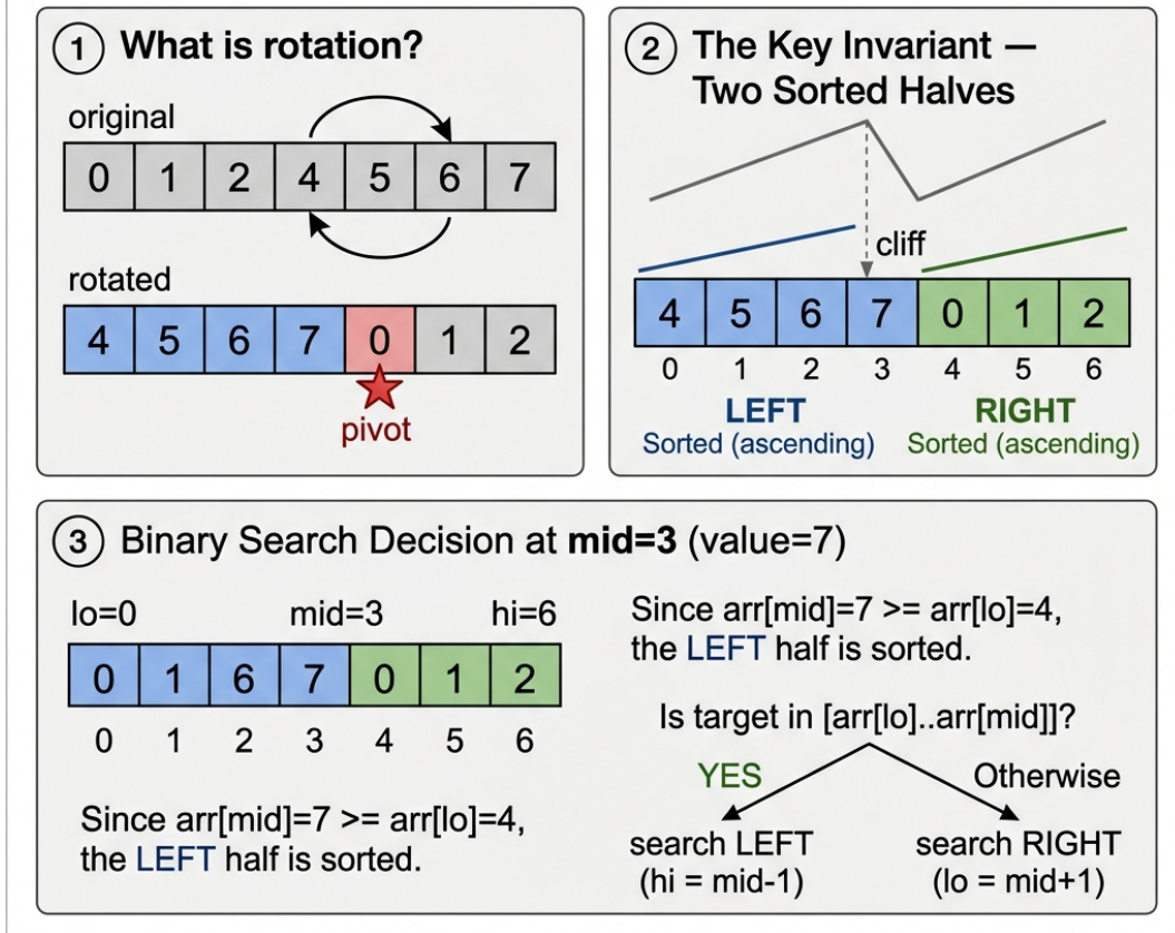
Figure 13.1: Binary Search on Rotated Sorted Array — Two Sorted Halves
