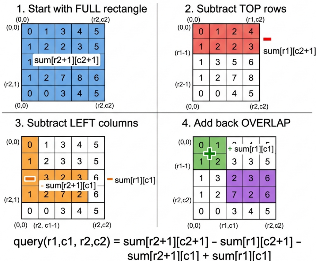
Figure 11.4: 2D Prefix Sum — Query via Inclusion-Exclusion
