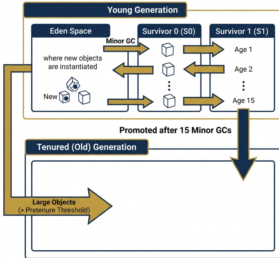
Figure 7.4: JVM Heap Generation Promotion Lifecycle
