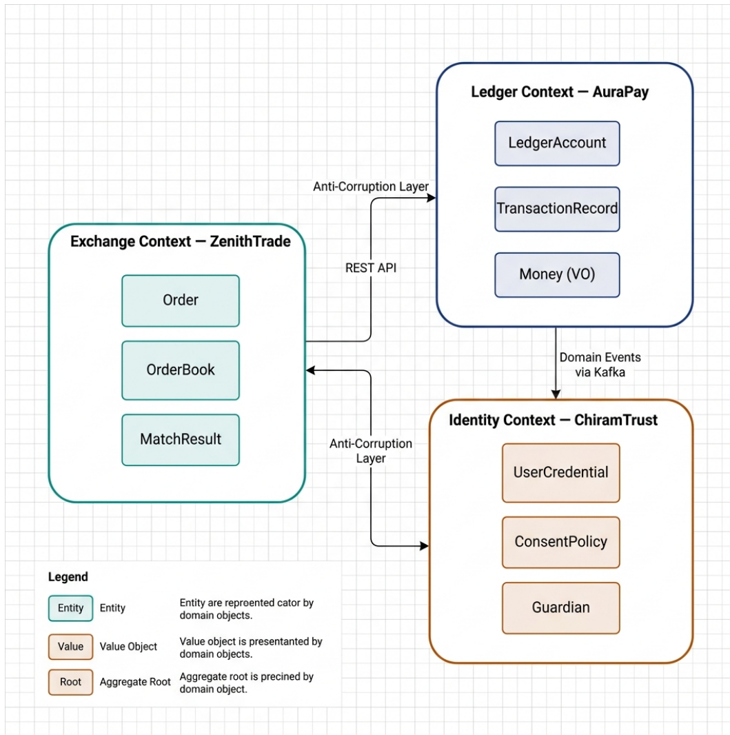
Figure 15.1: DDD Bounded Context Map
