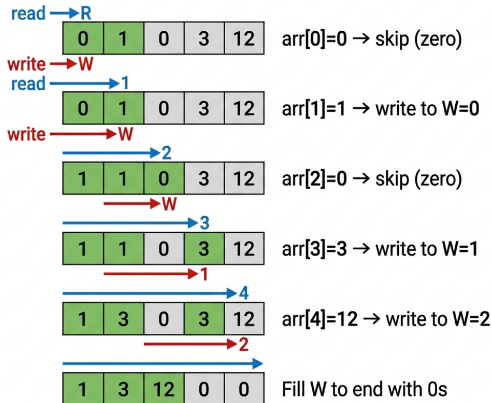
Figure 10.1: Read/Write Pointer — In-Place Array Compaction
