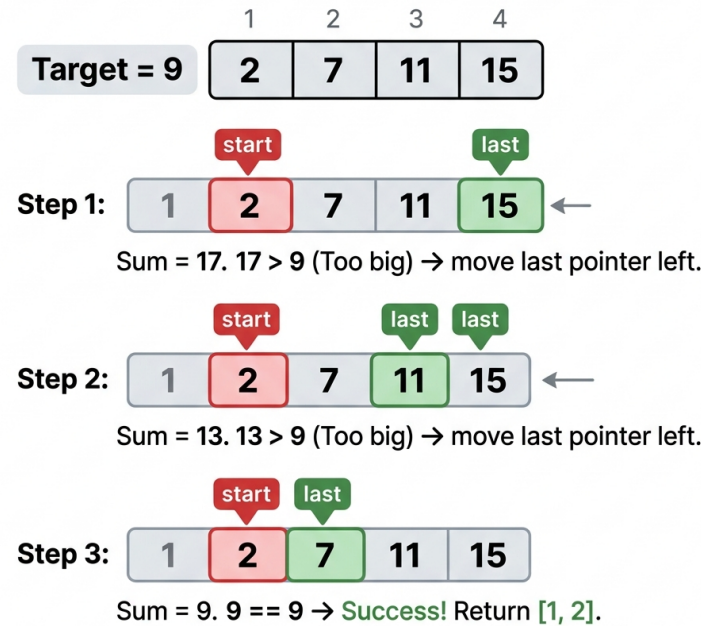
Figure 8.5: Two-Pointer Pattern — Two Sum Sorted Execution Trace
