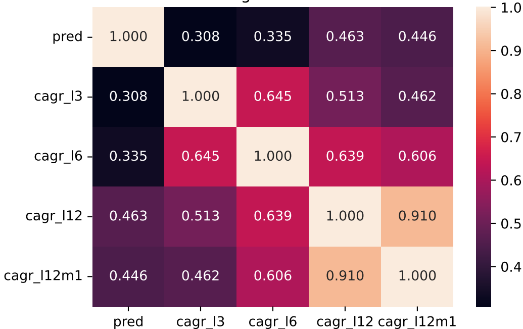
Correlation of return signals from xomRet for xomRet
