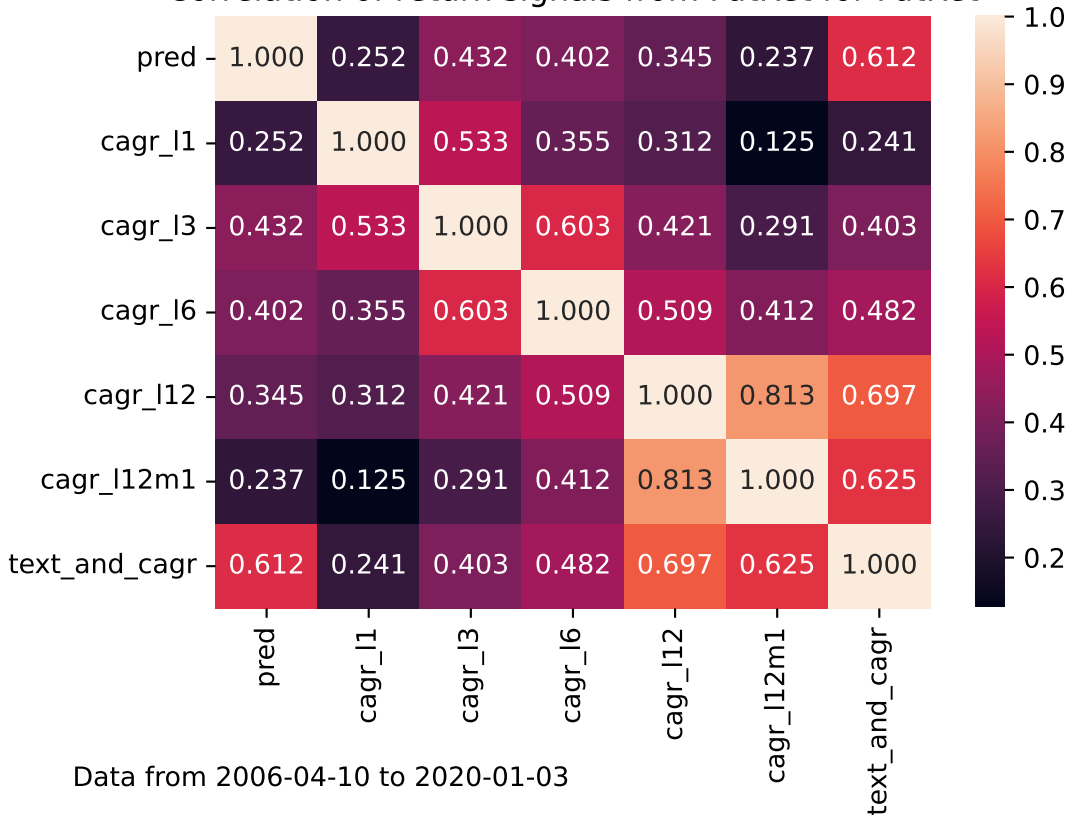
Correlation of return signals from FutRet for FutRet
