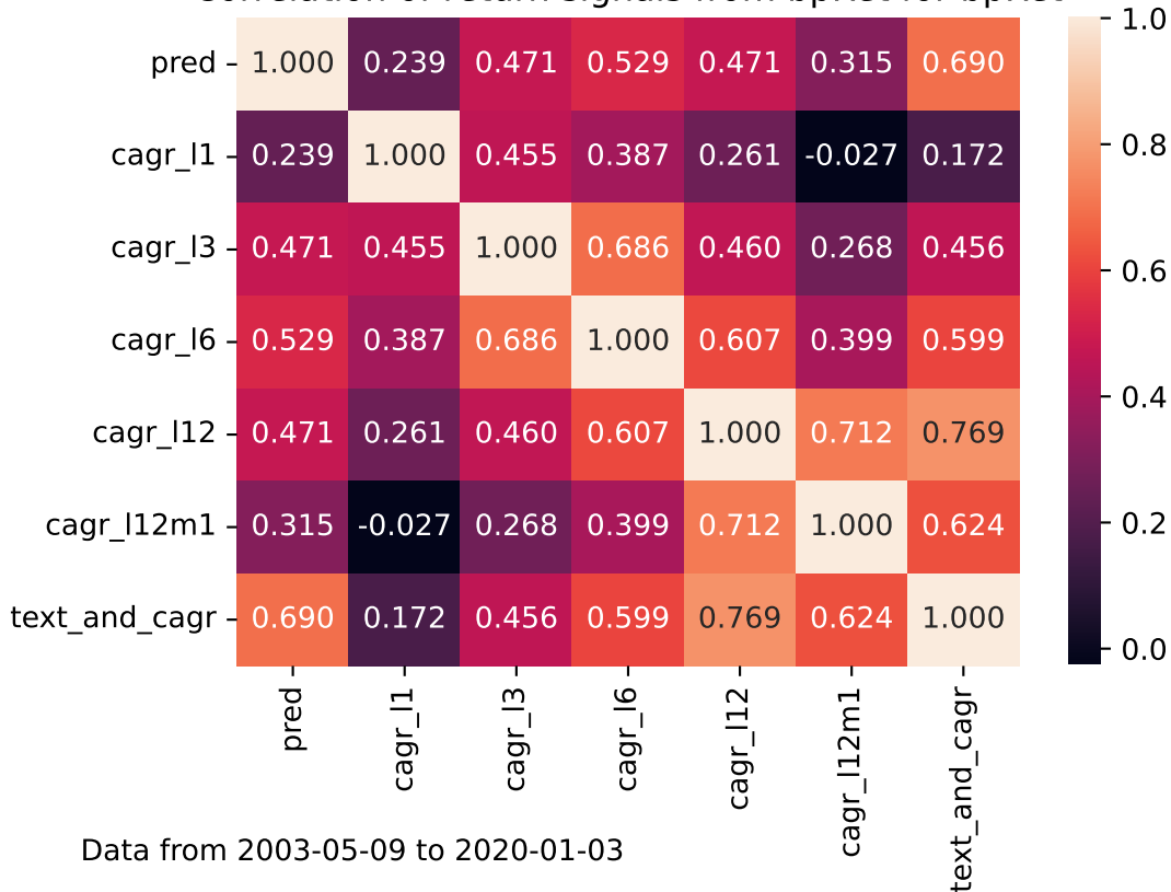
Correlation of return signals from bpRet for bpRet
