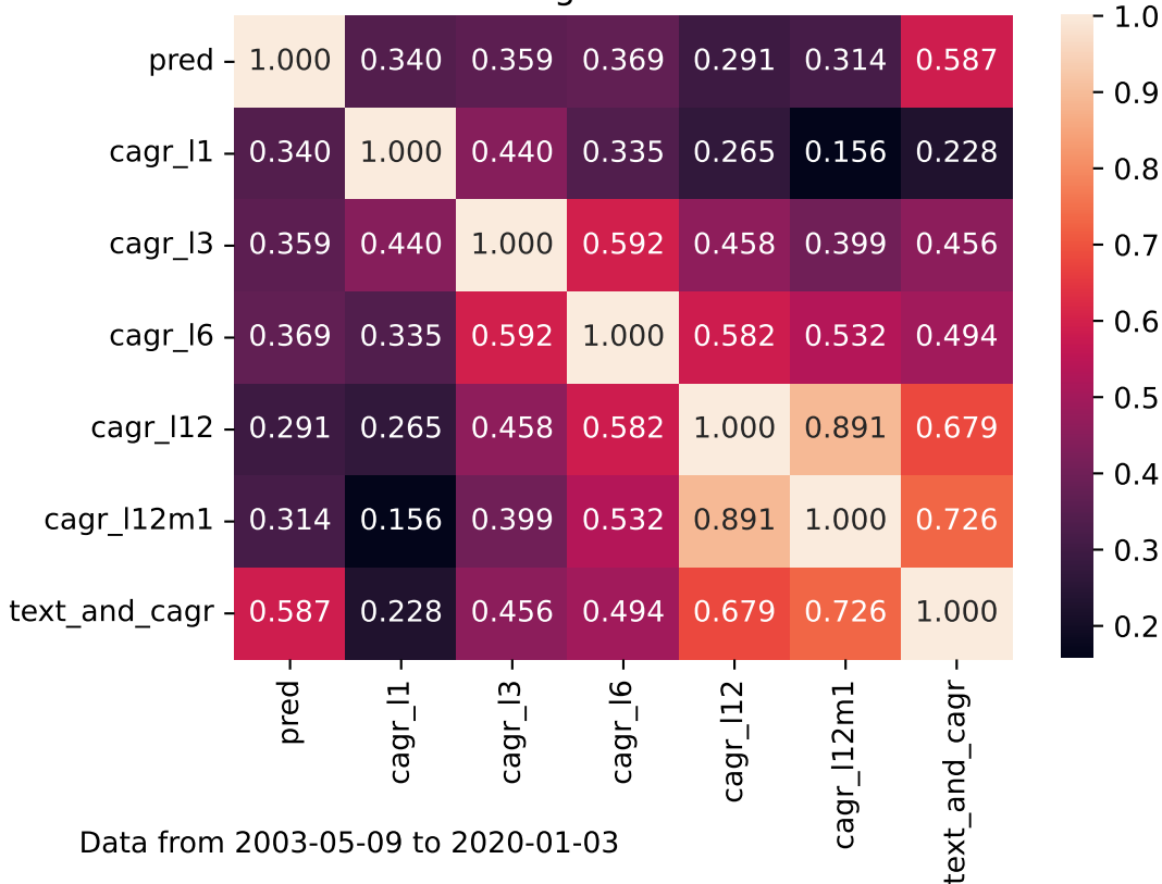
Correlation of return signals from rdsaRet for rdsaRet
