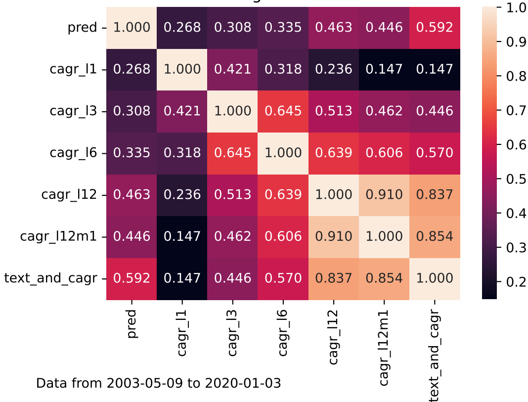
Correlation of return signals from xomRet for xomRet
