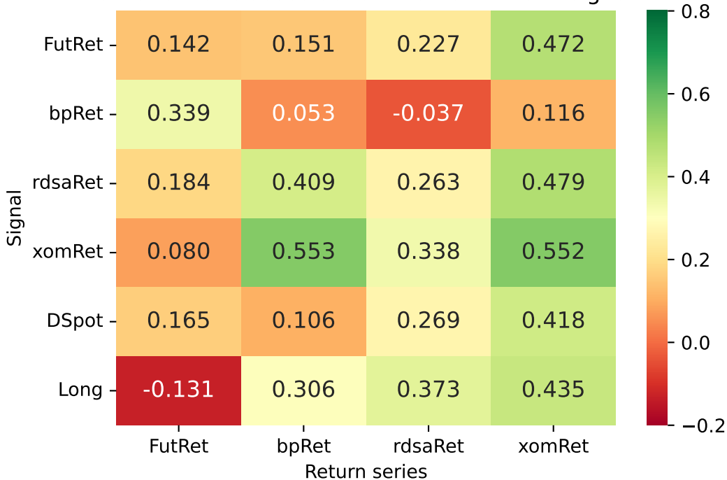
SR of asset classes as function of "mean" signal
