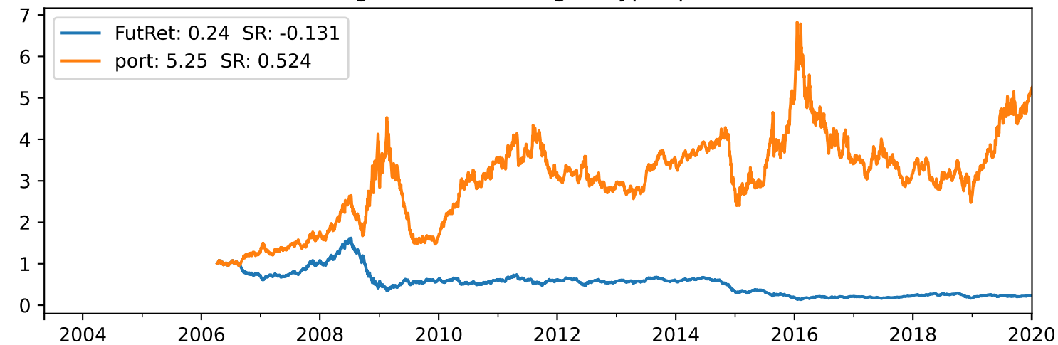
Cumulative excess returns for FutRet using FutRet signal "text" and signal type "pred"
