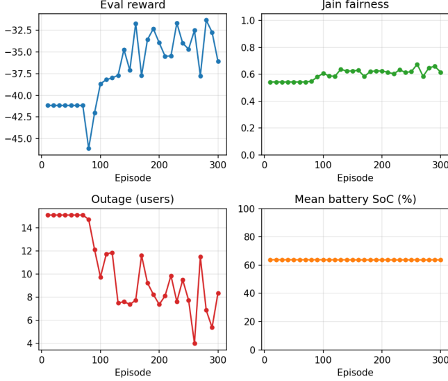
Fig. 11: DQN training convergence on the association MDP: evaluation reward, Jain fairness, outage, and mean battery SoC vs. training episode.
