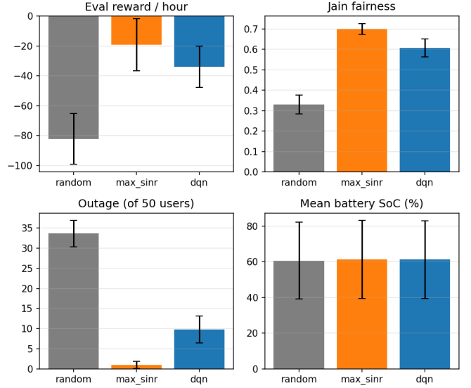
Fig. 12: Random vs. max-SINR vs. DQN, 50 held-out episodes (error bars: std).
