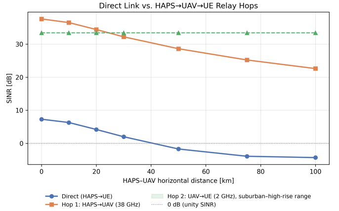
Fig. 6: Direct HAPS → UE SINR (suburban, averaged in dB over 24 azimuths, including co-channel interference from the other two HAPS) vs. the two UAV relay hops, as a function of HAPS–UAV horizontal distance. The HAPS → UAV feeder hop (orange, including interference from the other HAPS, which is about 35 dB below the noise floor) starts at +37.6 dB at nadir and stays above +22 dB at 100 km, well above the +8 dB design floor (Eq. (32)). The UAV → UE access hop (green, suburban and high-rise identical at 500 m) is +33.4 dB. The direct link falls from +7.3 dB at nadir to −9.1 dB at 100 km.
