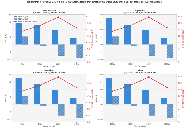
Fig. 9: 2 GHz service link SINR, four identical landscape subplots (landscape-independent, §III.C), 10–100 km distances.
