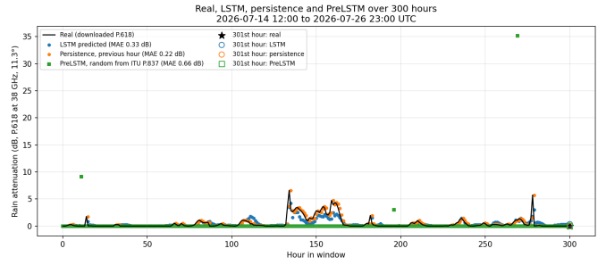
Fig. 11: Real, LSTM, persistence and PreLSTM over a 300-hour window in July 2026, the window with the most rain. Real: observed hourly attenuation from the downloaded precipitation (P.838 and P.618 method, gateway geometry). LSTM: one-hour-ahead forecast. Persistence: previous hour's value. PreLSTM: random hourly rain rates drawn from the ITU-R P.837 statistics for Delhi, converted with P.618; this is a synthetic baseline with no observed data. Star and open markers show the 301st hour.
