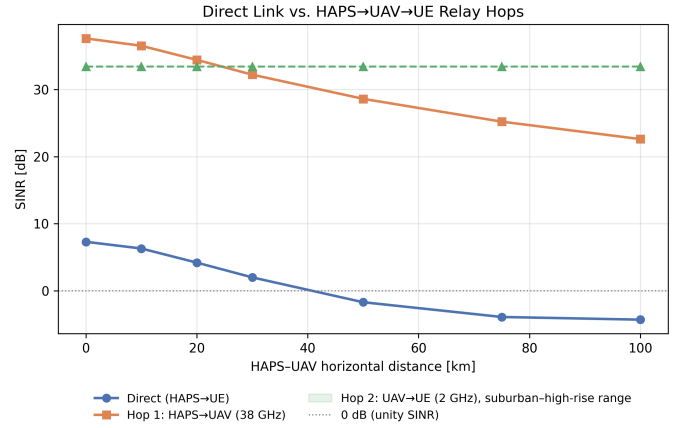
Fig. 6: Direct HAPS \rightarrow UE SINR (suburban, averaged in dB over 24 azimuths, including co-channel interference from the other two HAPS) vs. the two UAV relay hops, as a function of HAPS–UAV horizontal distance. The HAPS \rightarrow UAV feeder hop (orange, including interference from the other HAPS, which is about 35 dB below the noise floor) starts at +37.6 dB at nadir and stays above +22 dB at 100 km, well above the +8 dB design floor (Eq. (33)). The UAV \rightarrow UE access hop (green, suburban and high-rise identical at 500 m) is +33.4 dB. The direct link falls from +7.3 dB at nadir to -9.1 dB at 100 km.
