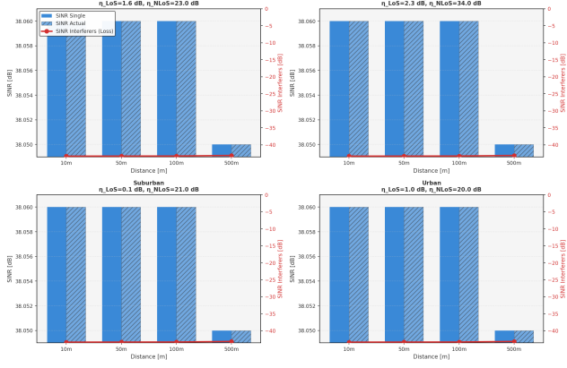
Fig. 10: 38 GHz backhaul link (HAPS-to-Gateway) SINR, four identical landscape subplots (landscape-independent, §III.C), 10–500 m distances.
