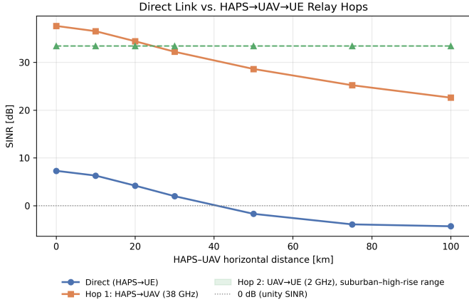
Fig. 7: Direct HAPS→UE SINR (suburban, averaged in dB over 24 azimuths, including co-channel interference from the other two HAPS) vs. the two UAV relay hops, as a function of HAPS–UAV horizontal distance. The HAPS→UAV feeder hop (orange, including interference from the other HAPS, which is about 35 dB below the noise floor) starts at +37.6 dB at nadir and stays above +22 dB at 100 km, well above the +8 dB design floor (Eq. (32)). The UAV→UE access hop (green, suburban and high-rise identical at 500 m) is +33.4 dB. The direct link falls from +7.3 dB at nadir to −9.1 dB at 100 km.
