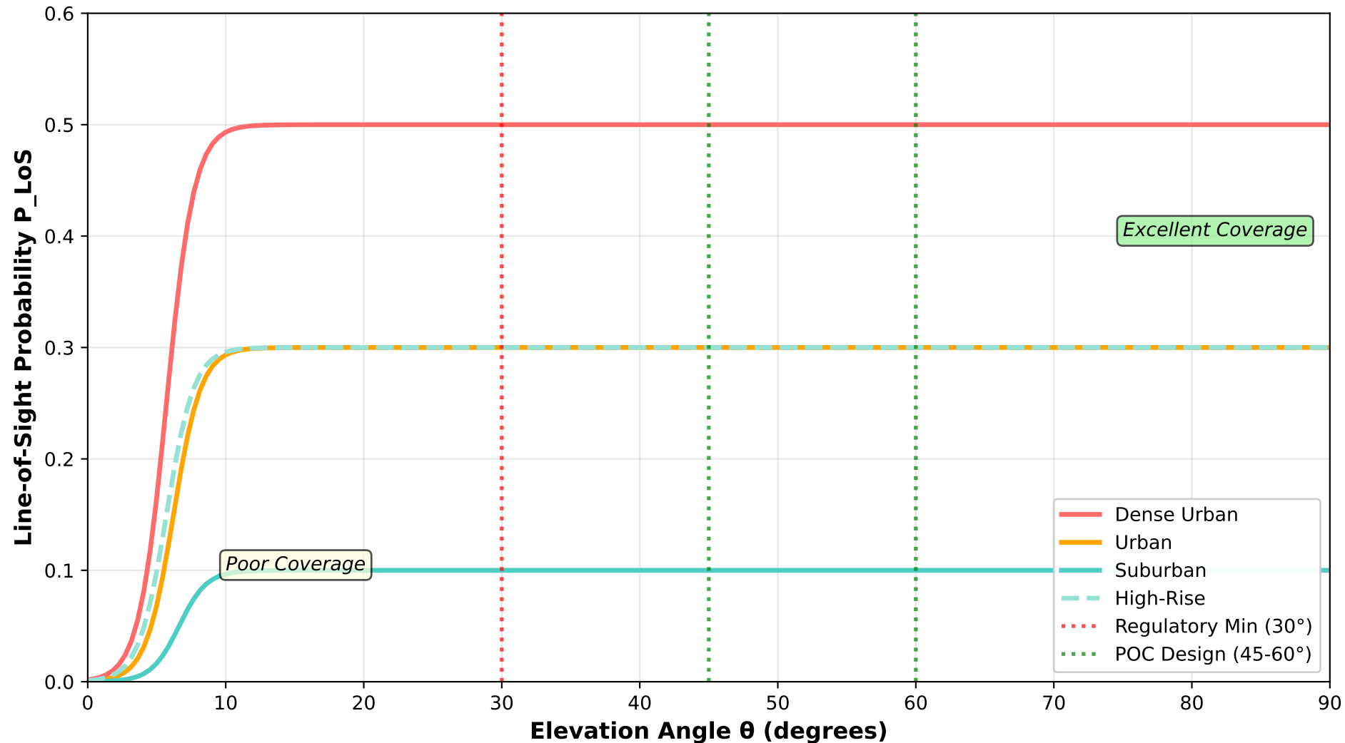
HAPS Elevation-Dependent LoS Probability (ITU-R P.1410)
