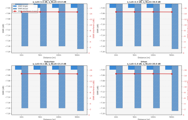
Fig. 9: 38 GHz feeder link (HAPS-to-Gateway) SINR, four identical landscape subplots (landscape-independent, §III.C), 10–500 m distances.
