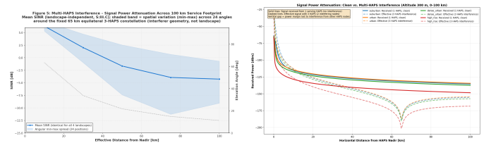
(a) Mean SINR and angular min–max spread across 100 km service footprint. (b) Received-power comparison showing clean vs. effective power under three-HAPS interference.
