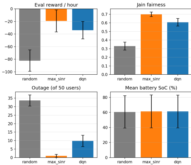
Fig. 11: Random vs. max-SINR vs. DQN, 50 held-out episodes (error bars: std.).
