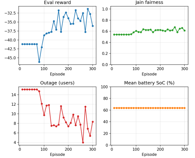
Fig. 10: DQN training convergence on the association MDP: evaluation reward, Jain fairness, outage, and mean battery SoC vs. training episode.
