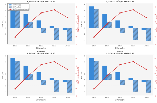
Fig. 8: 2 GHz service link SINR, four identical landscape subplots (landscape-independent, §III.C), 10–100 km distances.
