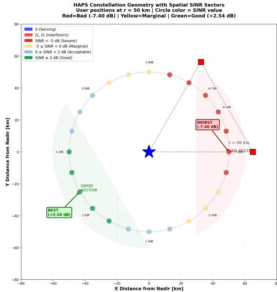
Fig. 6: HAPS constellation geometry (true 65 km equilateral triangle: S at origin, I1 at 0°, I2 at 60°) with spatial SINR sectors at r = 50 km. Good sector (green, away from interferers, \sim 120\text{--}290^\circ ) vs. bad sector (red, toward interferers, \sim 330\text{--}75^\circ ). Best +2.54 dB @ 210^\circ ; worst -7.40 dB @ 0^\circ .
