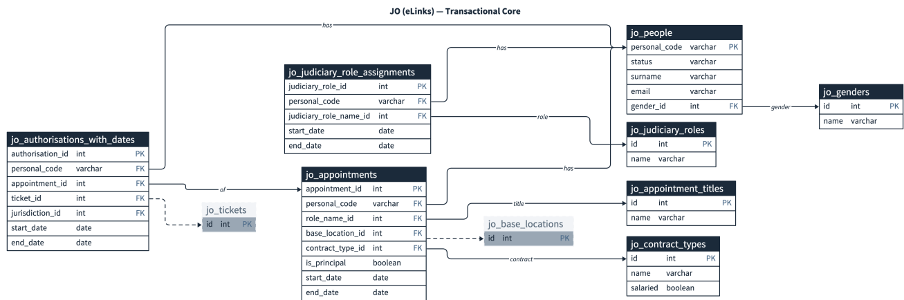
ER diagram — transactional core only
