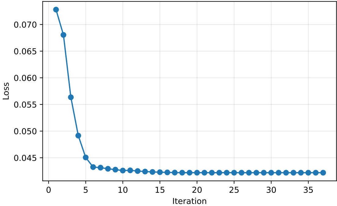
Loss curve | model=logistic, tying=5, agent=gpt-4.1-mini, prompt_category=numeric-certainty, domain=None, ver=2, temp=0.0
