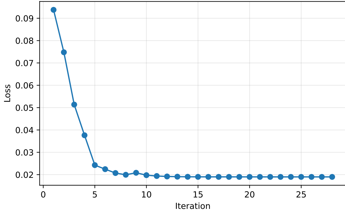
Loss curve | model=logistic, tying=4, agent=gpt-4.1, prompt_category=single_numeric_response, domain=None, ver=2, temp=0.0
